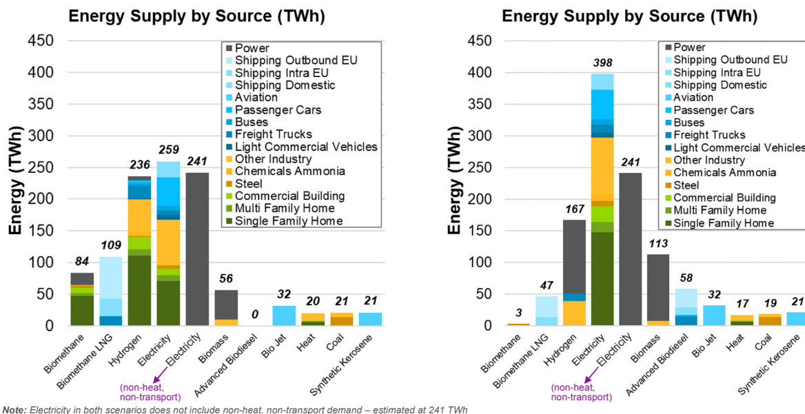
Figure 5 2050 Energy Supply by Scenario 14
