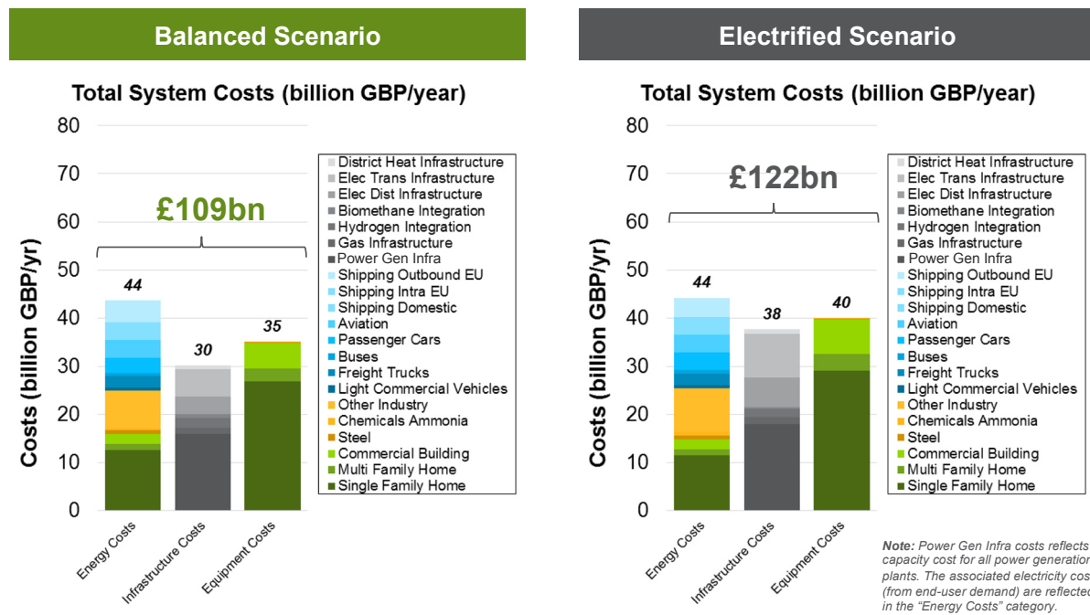
Figure 7 2050 Energy System Costs by Scenario
