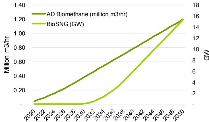
Figure 13 Biomethane production capacity along the Pathway
