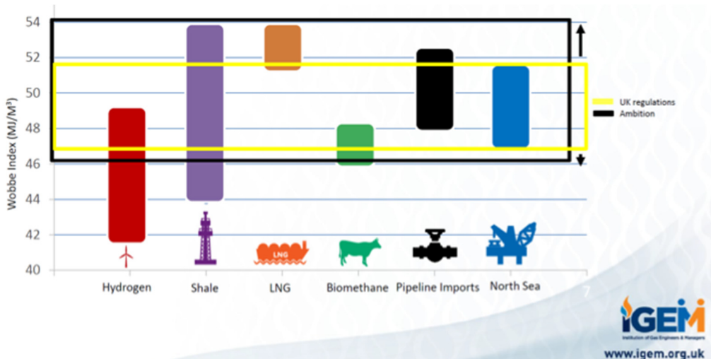
Figure 10 Drivers for a new GS(M)R standard. (Source: IGEM 21 )
